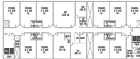
TYPICAL 3RD FLOOR CLASSROOM WING
